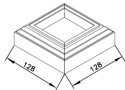
BASE PLATE INCLUDING COVER
