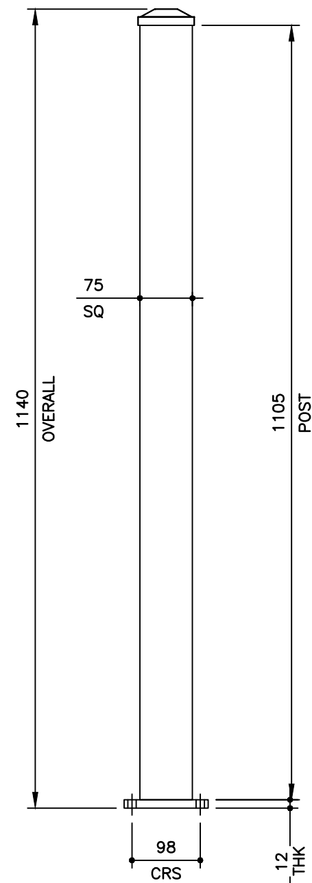
DETAILS OF POST
