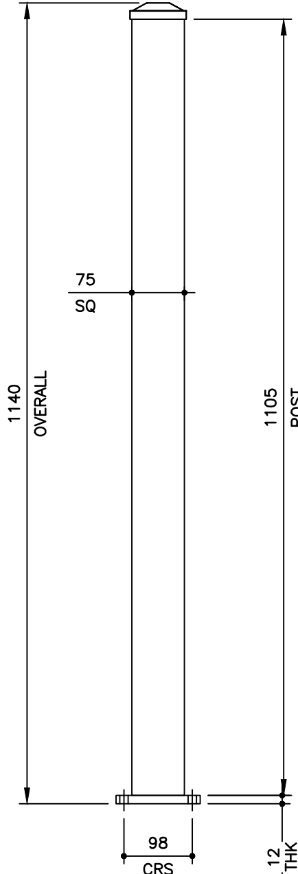
DETAILS OF POST
