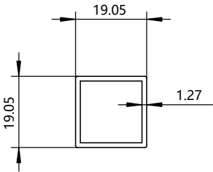
PICKET
