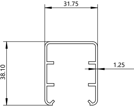
BOTTOM RAIL
