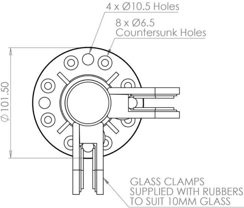
Base Plate Detail Scale 1:2
