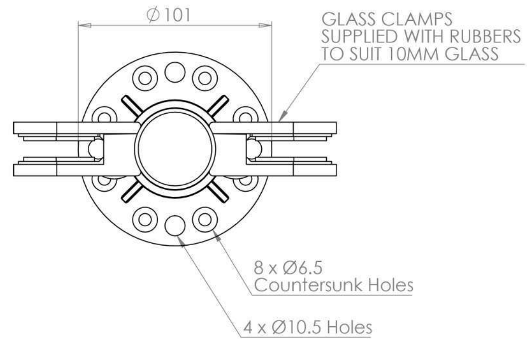
Base Plate Detail Scale 1:2
